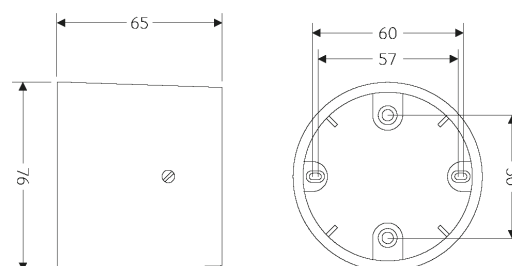
EBDBB - Surface mounting box
