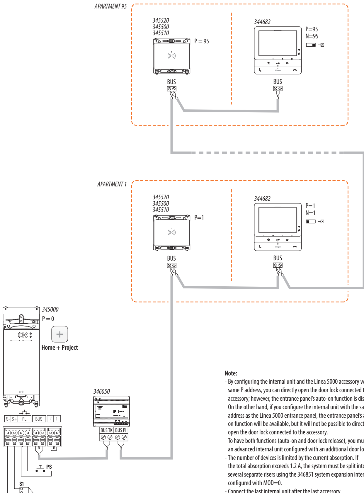
DIAGRAM 1 – EXAMPLE OF RESIDENTIAL SYSTEM FOR UP TO 95 APARTMENTS, WITH 1 ACCESSORY AND 1 INTERNAL UNIT FOR EACH APARTMENT
