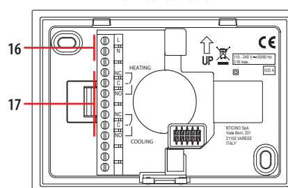
Wall mounted version
