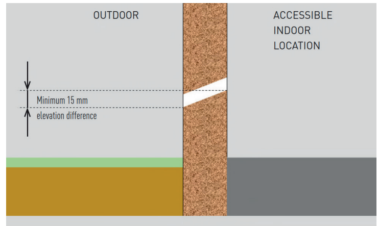
Cable entrance through exterior wall
