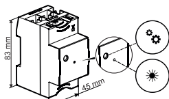
Funk-Gateway
