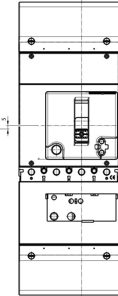
DPX 250 RCD
