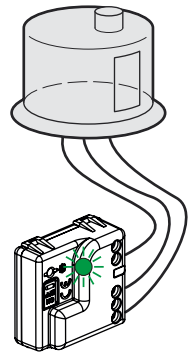
Connected switch without neutral 1 gang
