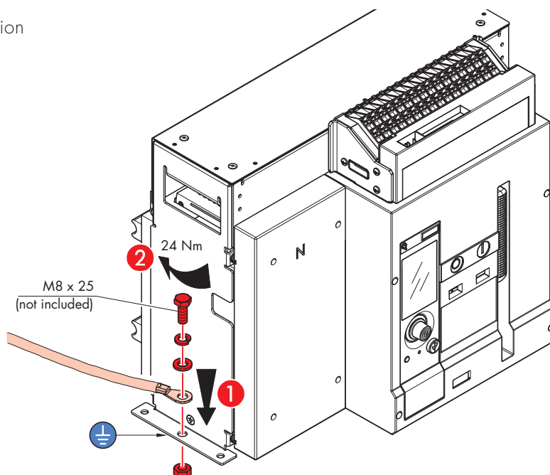
Draw-out version
