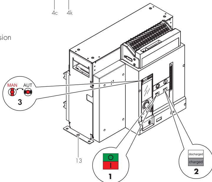
Draw-out version
