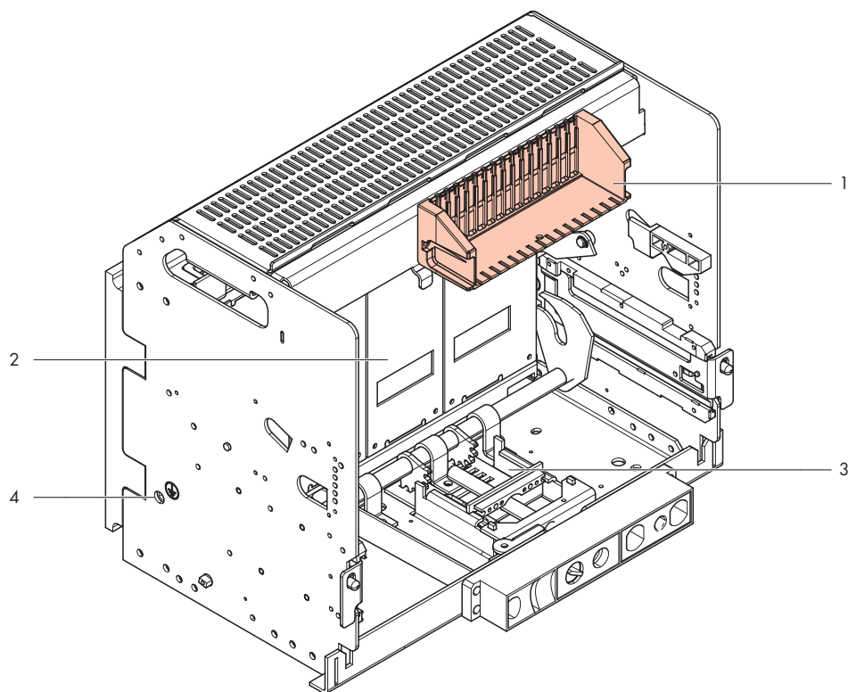
Draw-out version base
