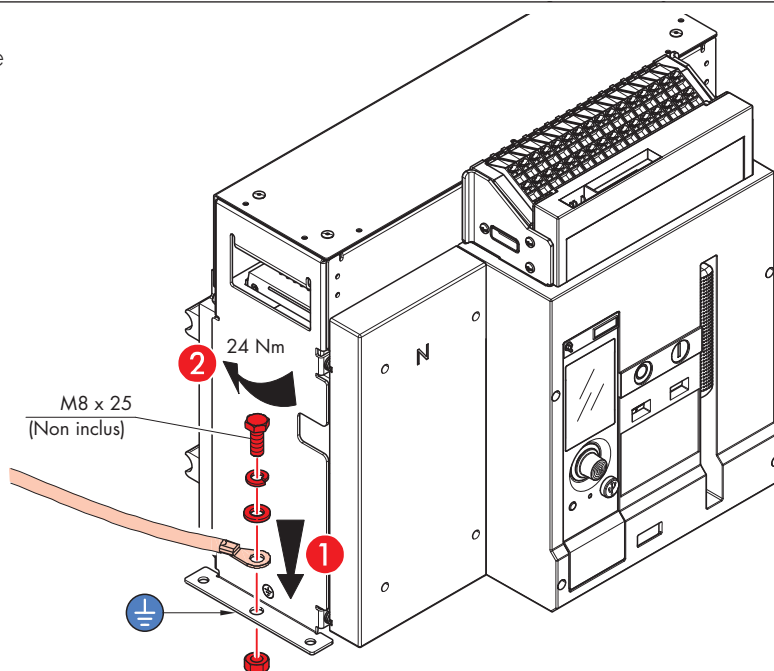
Version fixe
