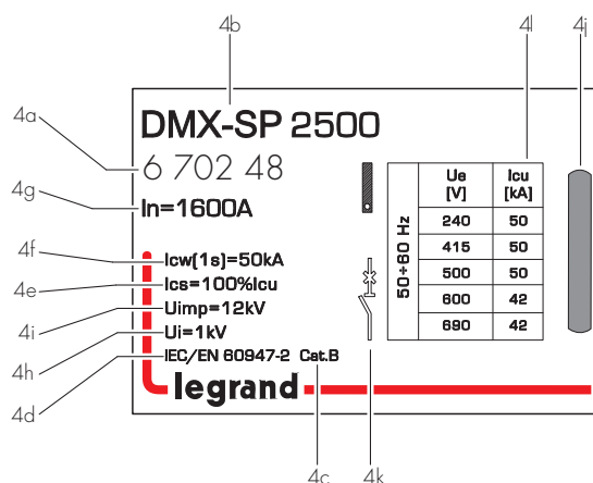
Fixed version
