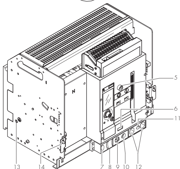
Draw-out version
