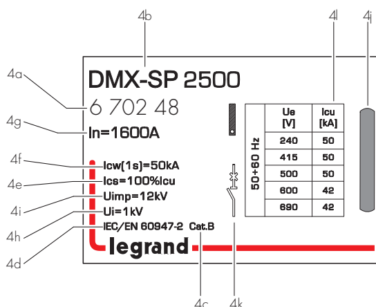
Version fixe
