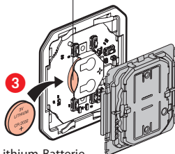
3-V-Lithium-Batterie CR 2032
