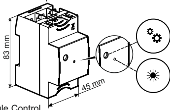
Module Control
