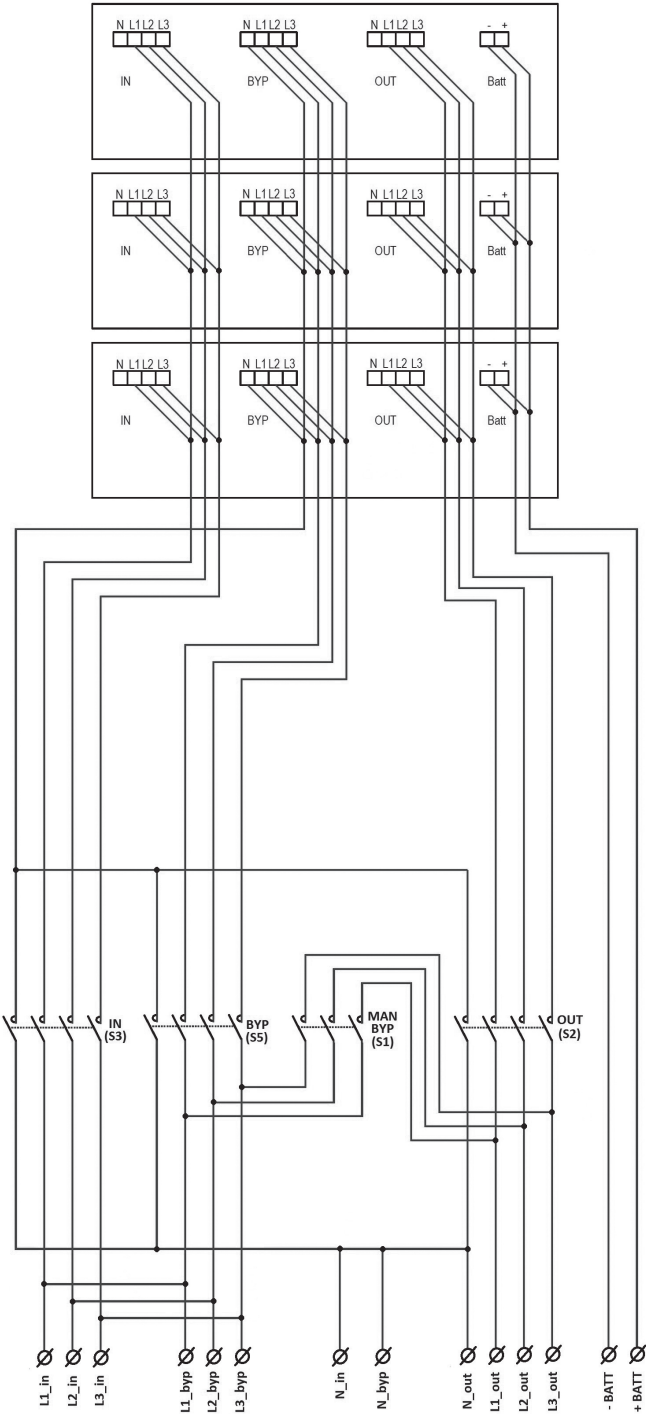
CABINET DISTRIBUTION
