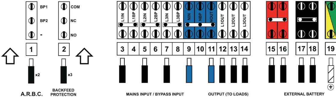
Trimod MCS 80
