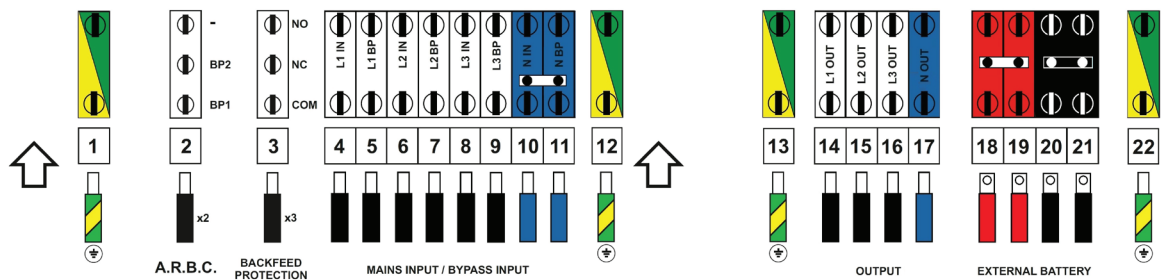
Trimod MCS 30
