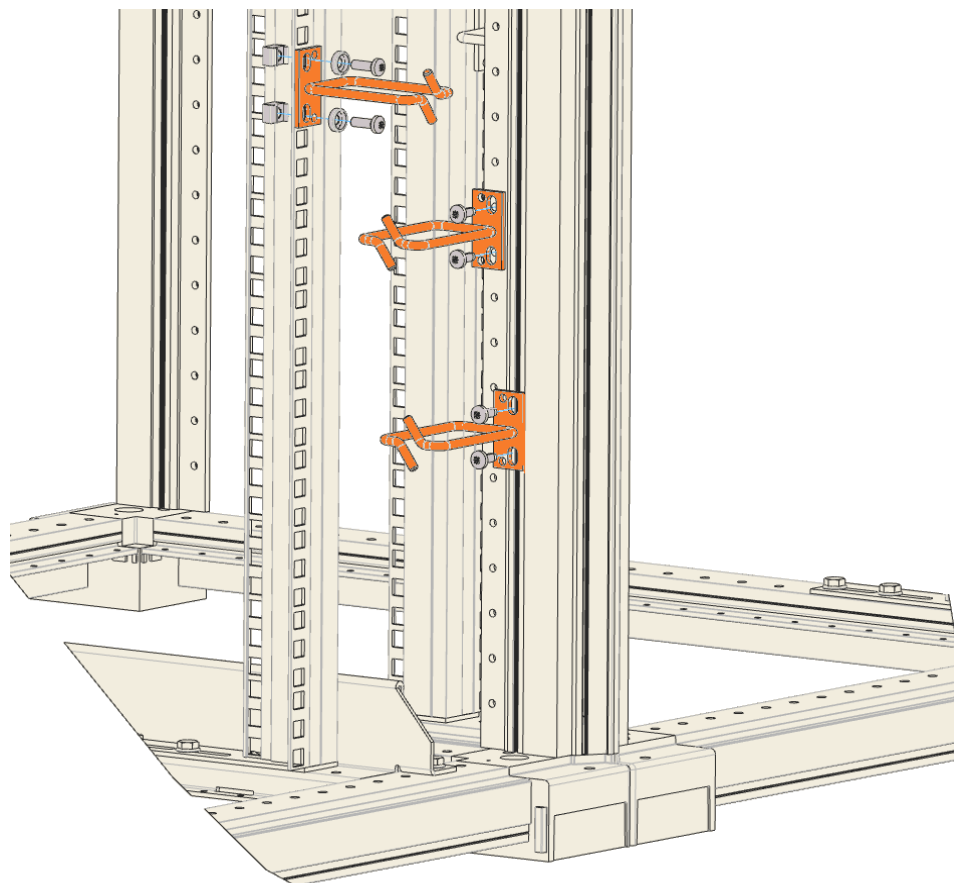
viewVue de face — Front view
