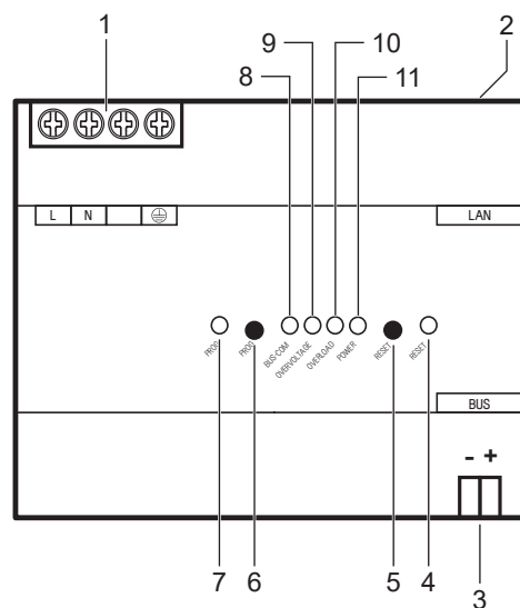
Fig. 1: Device components
