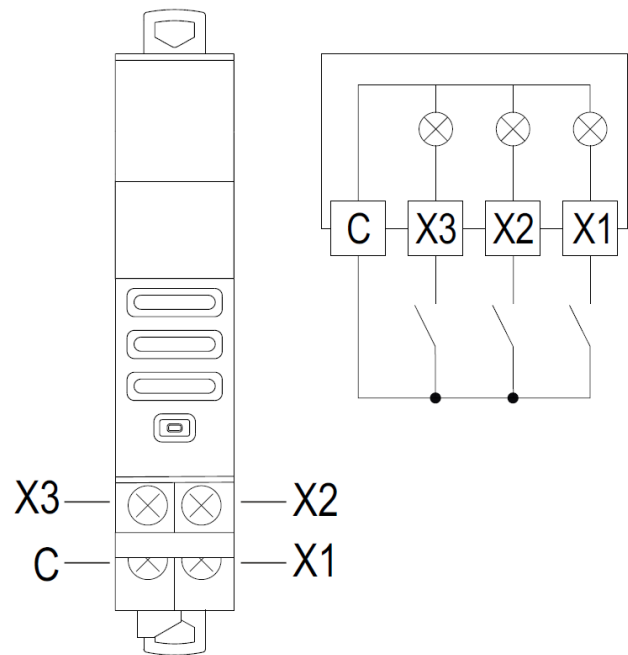
Inputs from voltage-free SPST NO contacts
