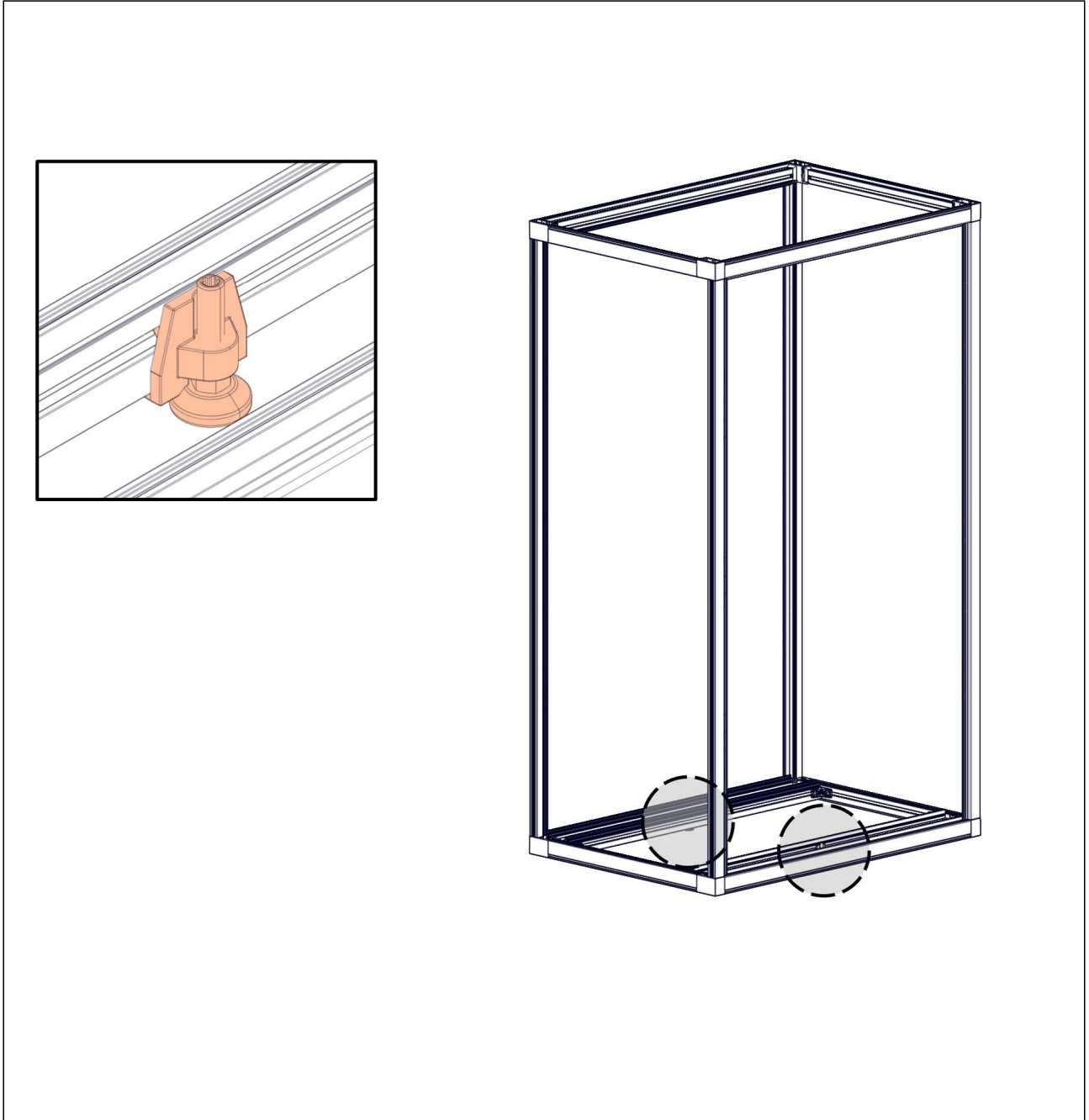
Cabinet Heavy load leveling feet
