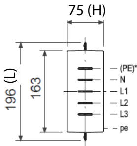
Section dimensions*
