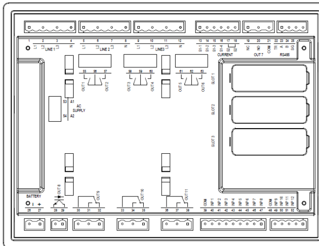
Rear connections
