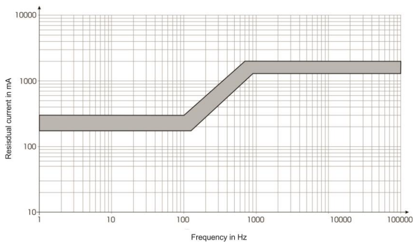
Tripping current frequency response 300 mA
