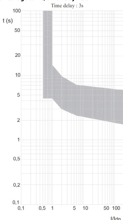
■ 9.7 Earth leakage curve, time delay = 3 s
