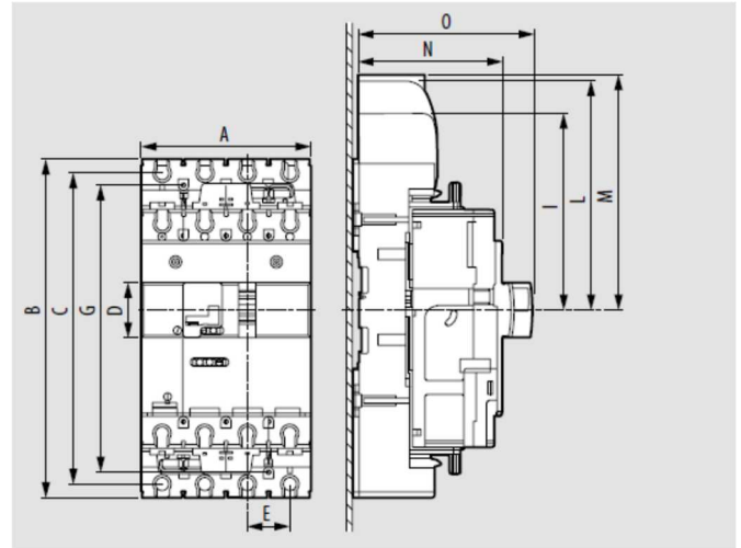
Plug-in version
