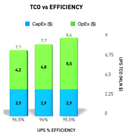
Correlation between TCO and efficiency
