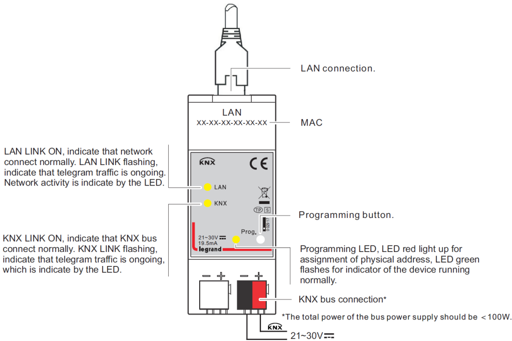
Fig. 3.2.1 Connection diagram
