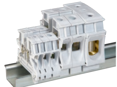
Same profile up to 10 mm pitch and same height from 12 to 22 mm pitch
