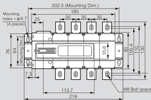
Frame 1, 4-pole, Cat.Nos 4 241 13/14/15
