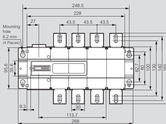
Frame 2, 4-pole, Cat.Nos 4 241 23/24/25
