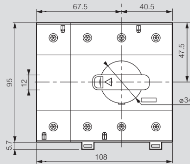
Frame 2, 3P+N with Cat.Nos 4 242 19/20/21
