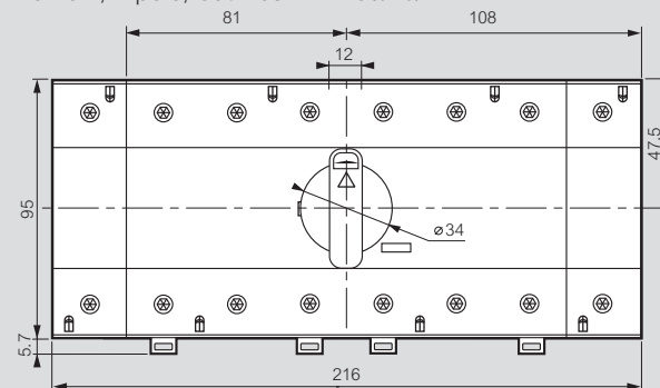
Frame 2, 4-pole, Cat.Nos 4 241 09/46/47
