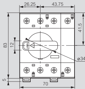
Frame 1, 3P+N with Cat.Nos 4 242 04/05/06
