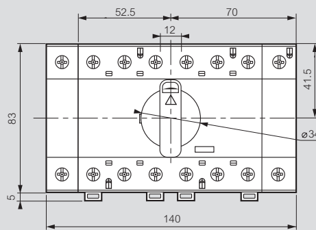
Frame 1, 4-pole, Cat.Nos 4 241 06/07/08
