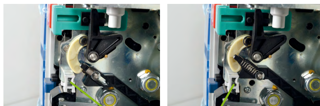
Wedge stop
