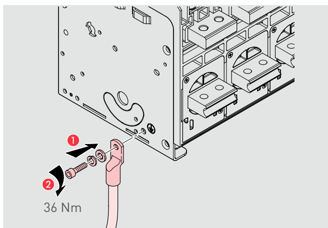
Fixed version
