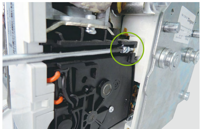
Fix the 2nd motor operator holding screw (Phillips head n°2, tightening torque 3 Nm).
