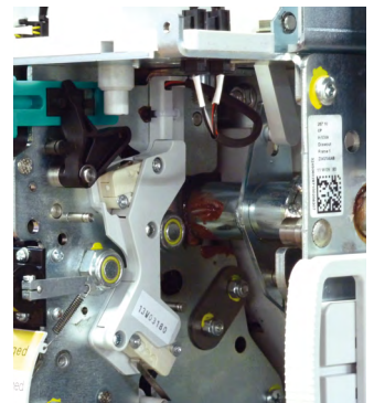
Contact block mounted inside the DMX-SP
