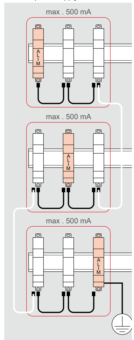
1 EMS CX 3 system 3 power supply modules
