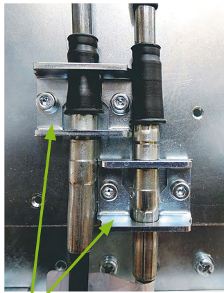
Locking flanges
