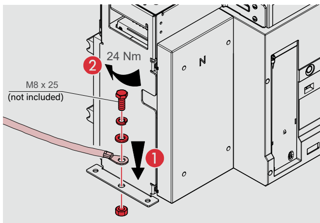
Fixed version
