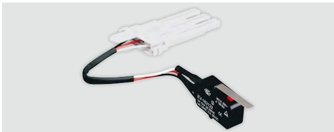
i OC : Open Close → auxiliary contact state
