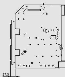
Flat terminals 4P
