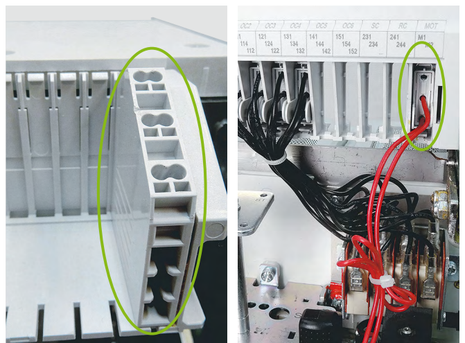
Clip the connector and terminal block into the dedicated slots: here MOT (M1/M2).
