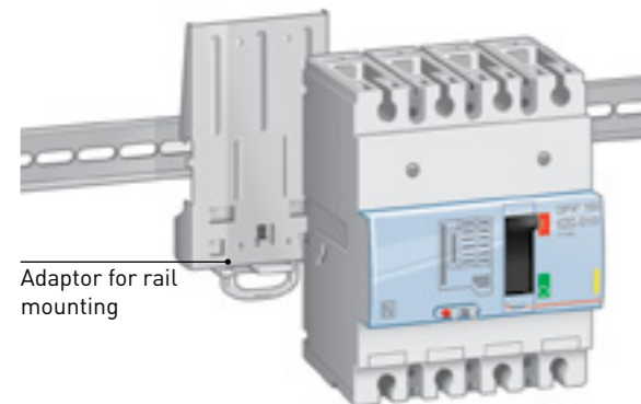
Mounting a DPX 3 160 on a rail
