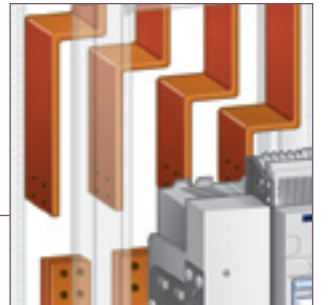
DMX 3 connection kit
