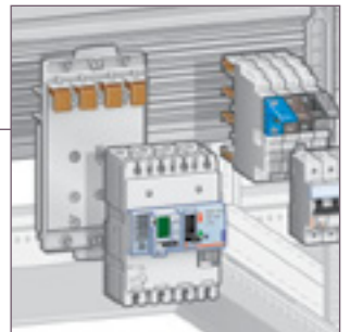
DPX 3 and modular devices together on the same row
