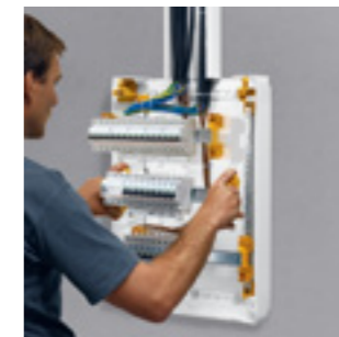
Tool-free removable rail Rails can be removed individually in a single movement, and without any tools, for easier cable routing
