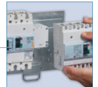
Easy to install: mounting on front panel with no adjustment
