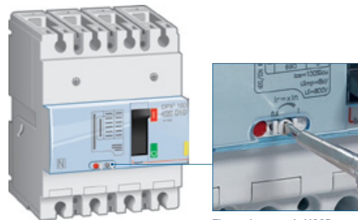
Thermal-magnetic MCCBs are adjusted on the front panel using a screwdriver
