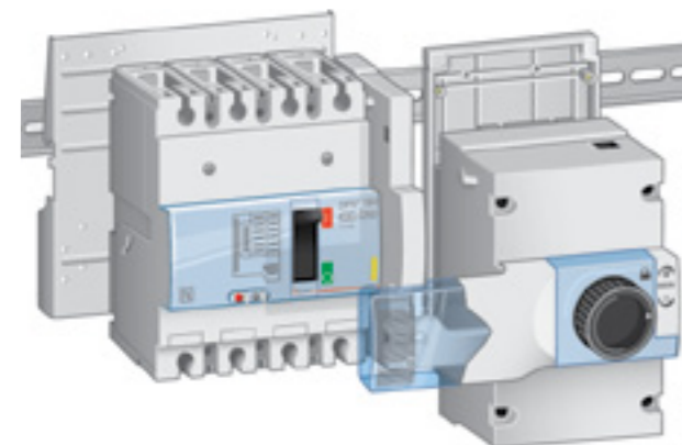
Mounting a DPX 3 160 with side motorised control on a rail
