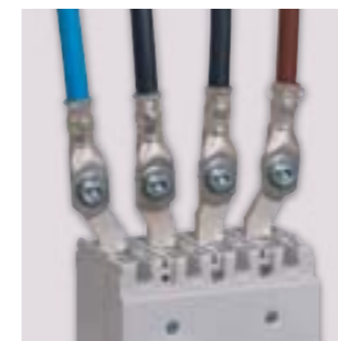
The spreaders enable connection via large cross-section cables
